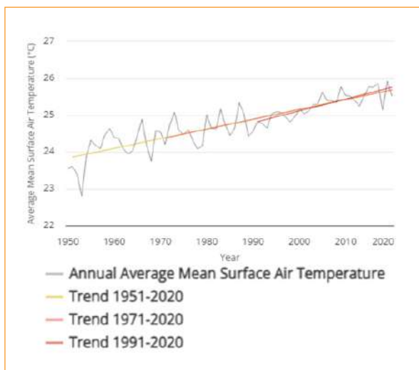
Figure 2b: Average mean surface air temperature annual and decadal trends 1950-2020 in Kenya
